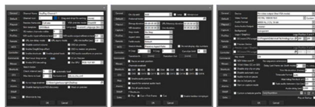
GENERAL SETTINGS
